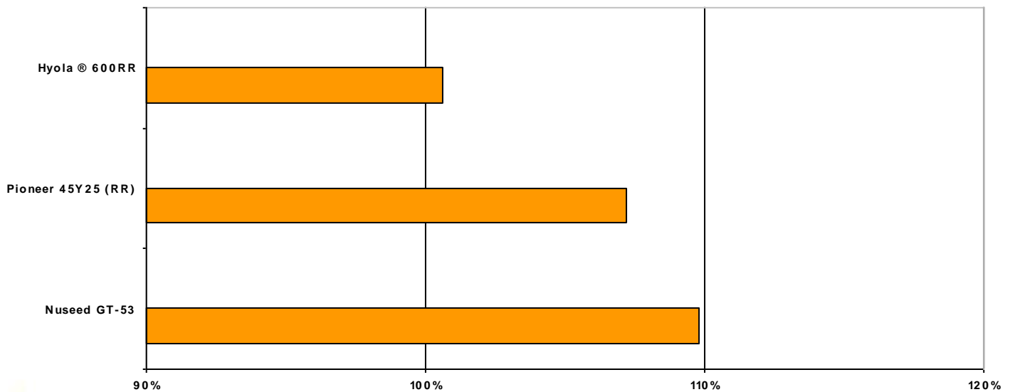
Average Variety Trial Yield Against Average Trial Yield Mean
